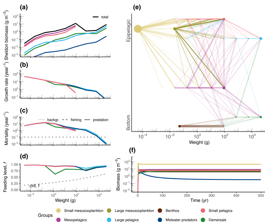
FIGURE 2 Main FEISTY outputs using the Vertical2 set-up with a seafloor depth of 800 m, a mesozooplankton productivity of 80 g WW m -2 year -1 , and no fishing. (a) Normalized 'Sheldon' biomass spectrum (g m -2 ; see Box V in Andersen and Visser (2023)), (b) growth rate (energy invested in growth, year -1 ), (c) total mortality \mu (year -1 ) and (d) feeding level f (consumption relative to maximum consumption, dimensionless), with the dotted line showing metabolic requirements (critical feeding level). (e) Illustration of the food web. Circle areas scale with the biomass of each size class, while line width, representing the feeding flux level between prey and predator, scales with the cube root of the feeding flux. (f) Convergence of the total biomass of each functional type. These plots are provided in the Shiny app webFEISTY().
